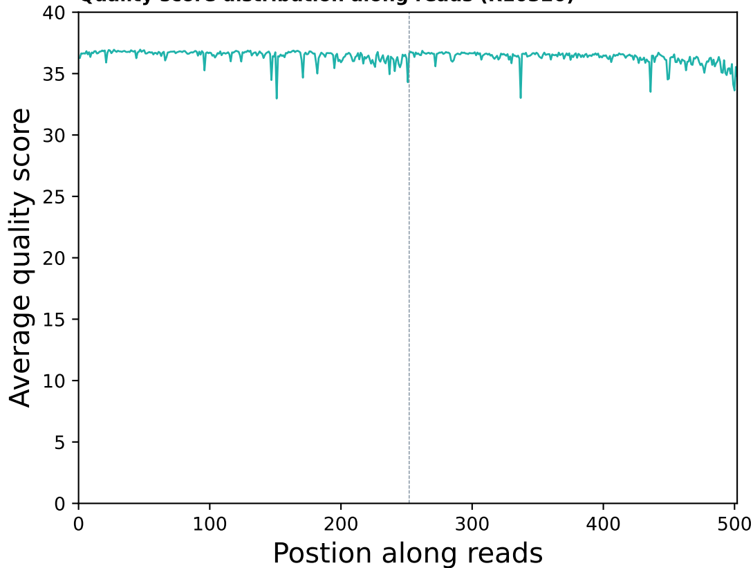
Quality score distribution along reads (R10320)
